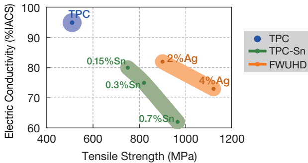
【導電率と引張強度】 Tensile Strength and Electric Conductivity at \phi 0.06 \text{ mm (H)}
