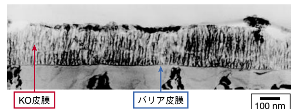
図1 KO処理皮膜の断面TEM像 TEM image of the KO processing film.
