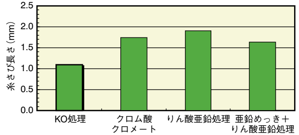
図5 各種処理材の糸さび試験結果 Results of filiform corrosion test of KO and other surface treatments.
