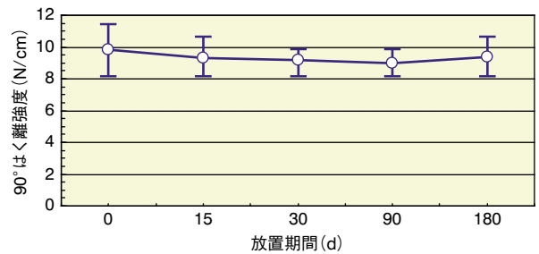
図6 KO処理板の90°はく離強度の経時変化 Change in 90° peeling strength of KO processing sheets over exposure time in humid atmosphere.
