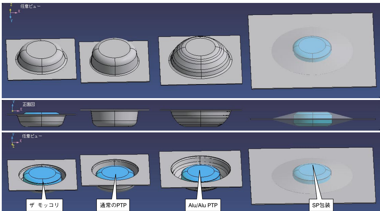
図5 ザ モッコリの形状比較(上段:底面, 中段:側面, 下段:上面) Comparison of THE MOCCORI with other PTPs. Upper line: bottom face, Middle line: side face, Lower line: top face.
