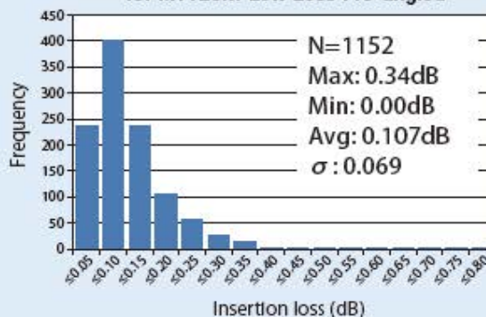
Insertion loss @1310nm for MT12SM-Low Loss Pre-angled
