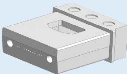
MT Ferrule (12SM-Low Loss Pre-angled)
